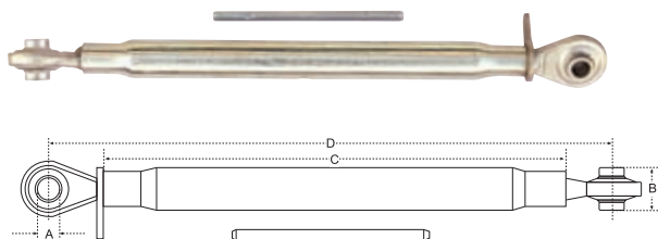
Tercer punto estandar Top link assembly, metric-light duty 62TLR0226 - 62TLR0266
