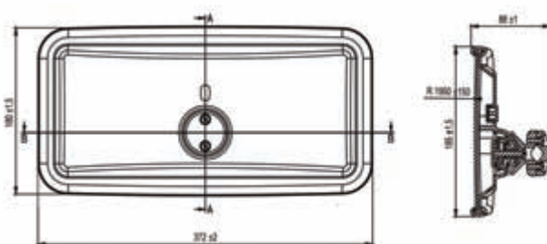
Ref. 16375185180 - Varilla Ø16mm / Mirror bracket arm Ø16 mm 375x185 mm - Curvo / Curved mirror
