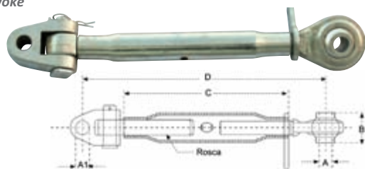
Tercer punto Articulado Top link assembly, with articulated yoke
