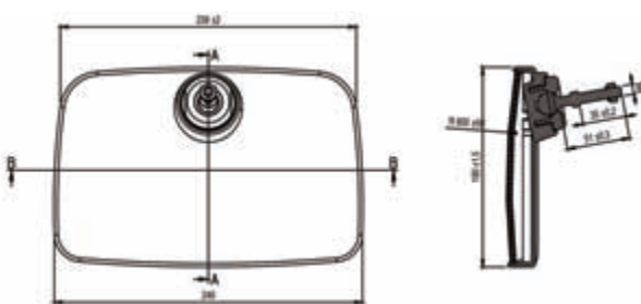
Ref. 16250140150 - Con rótula interior / with inside yoke 375x185 mm - Curvo / Curved mirror
