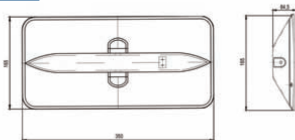
Ref. 16350165160 - Varilla Ø16mm / Mirror bracket arm Ø16 mm 350x165 mm - Curvo / Curved mirror
