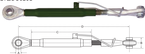
Tercer punto john deere John deere top link 62TLJDO0201
